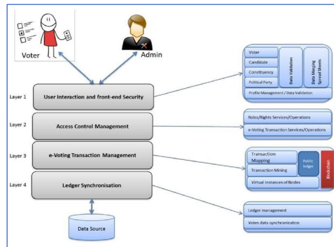
Figure 2 :: Architecture for proposed e-voting system
