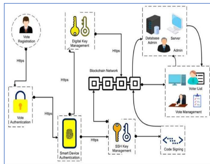
Figure 3 : Blockchain voting system architectural overview
